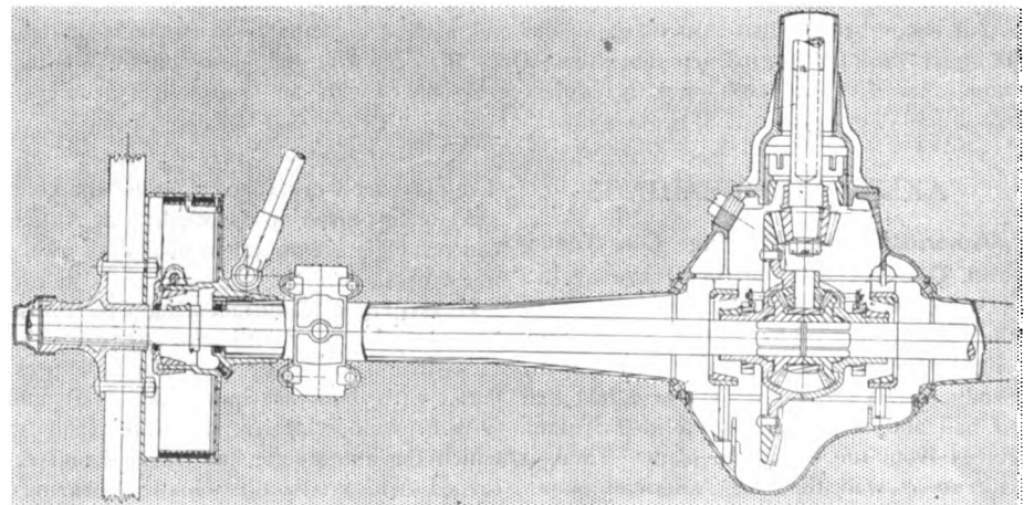
Timken Live Rear Axle—New 1,500-Pound Type.
